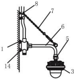
b1: 壁式90°
