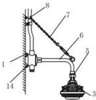
b1: 壁式90°
